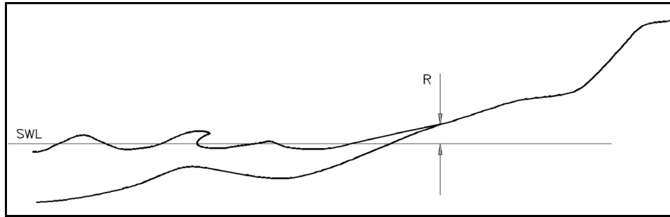
Figure II-4-11. Definition sketch for wave runup
