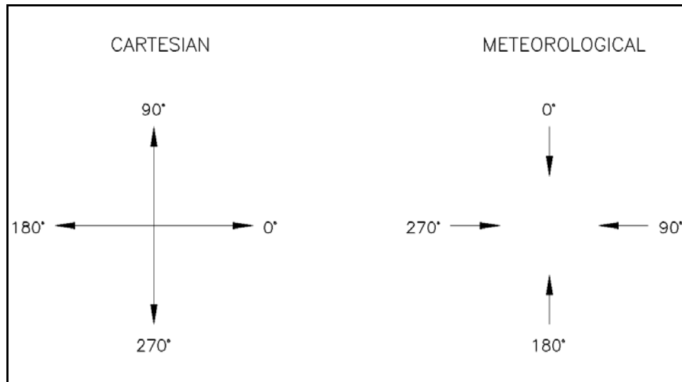
Figure II-2-15. Common wind direction conventions
