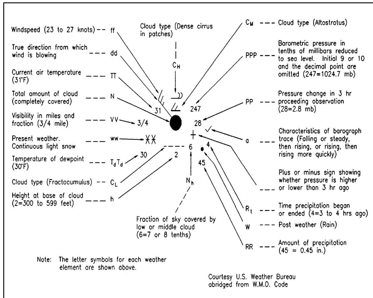
Figure II-2-11. Key to plotted weather report
