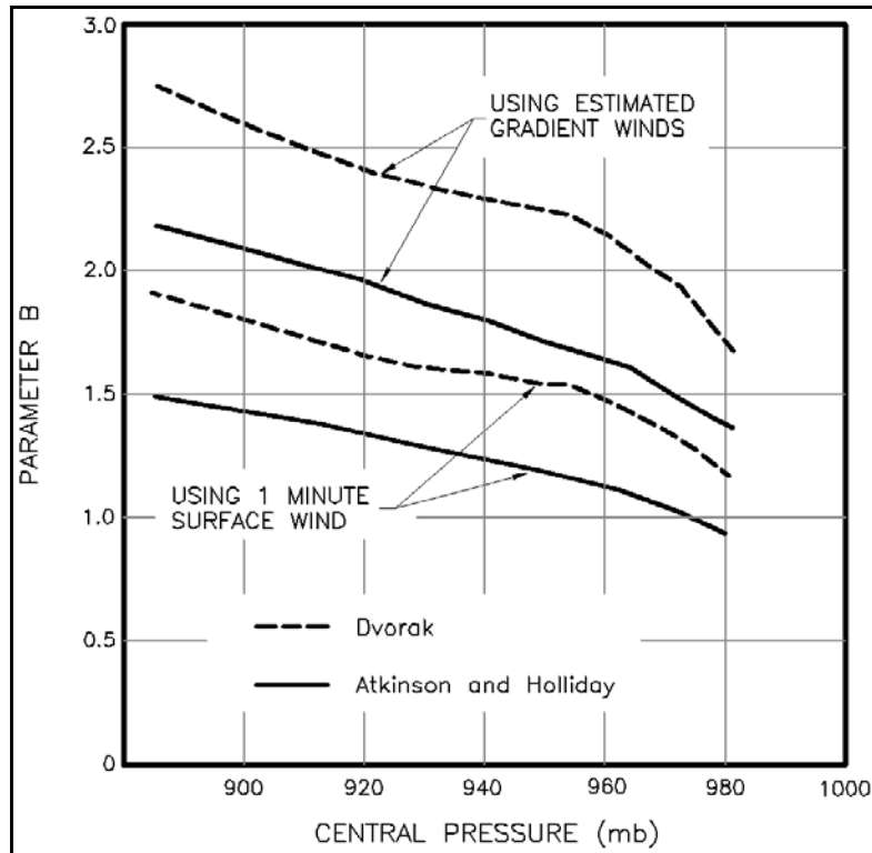
Figure II-2-16. Climatological variation in Holland's "B" factor (Holland 1980)
